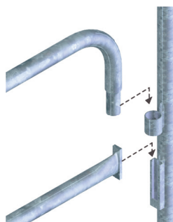
Single Entry Assembly
