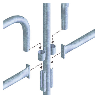
Double Entry Assembly
