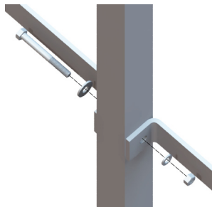
bolt together assembly
