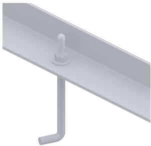
core drill and mix concrete to anchor J-Bolts
